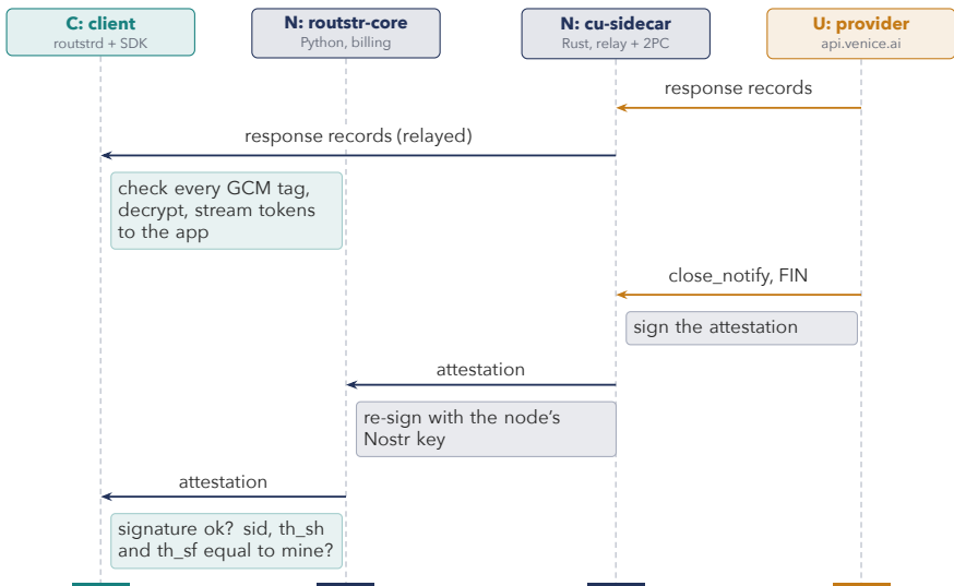
Figure 7.8: The response streams to the client; the node attests what it relayed.
