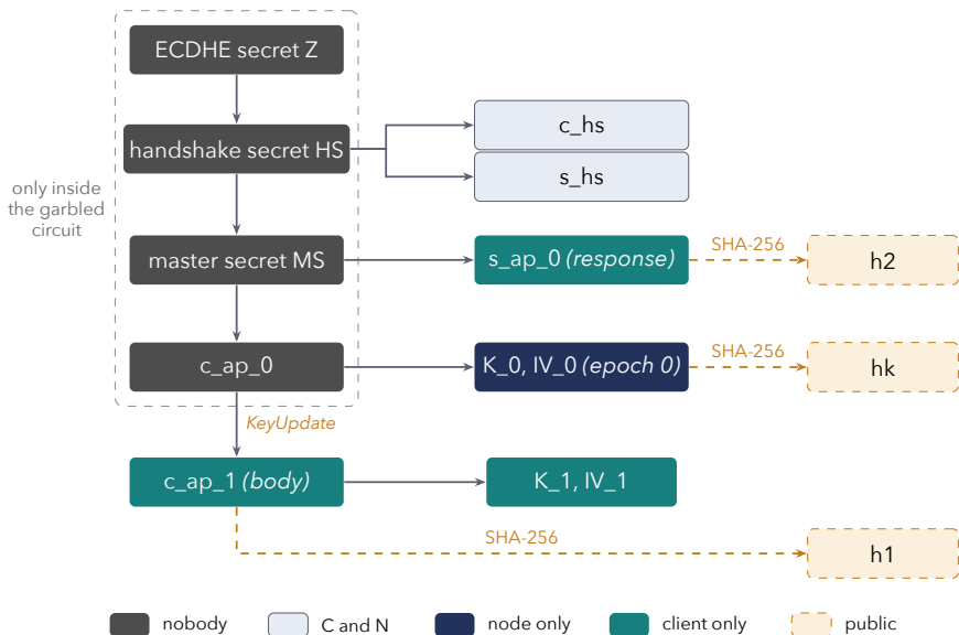
Figure 3.1: The TLS 1.3 key schedule, colored by who ends up holding each secret.
