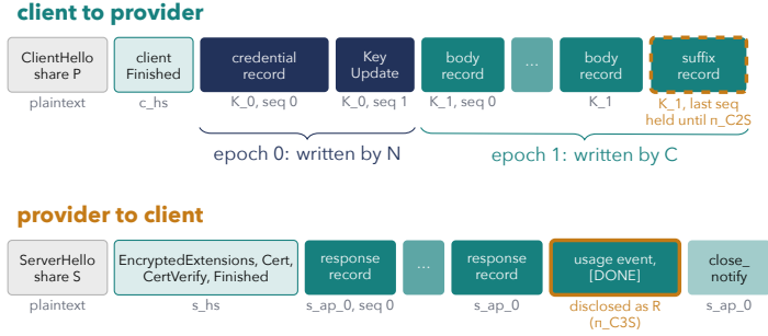
Figure 4.1: The records of one session as U sees them. The node writes only the two navy records.
