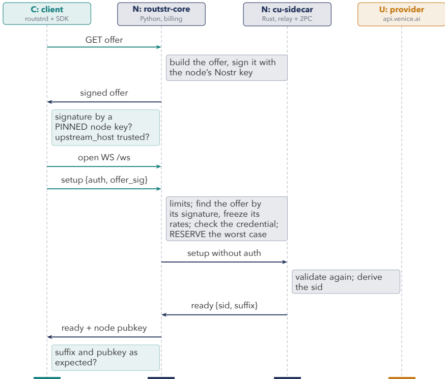
Figure 7.1: Setup: nothing is reserved before the credential checks, and the sidecar never sees the credential.
