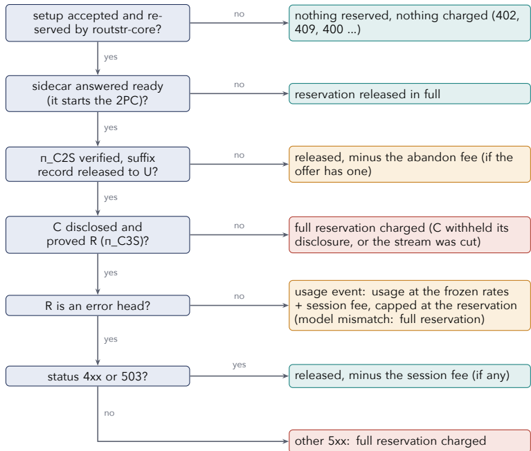
Figure 12.1: How a session's reservation ends. Teal: free, amber: fee or usage, red: full reservation.
