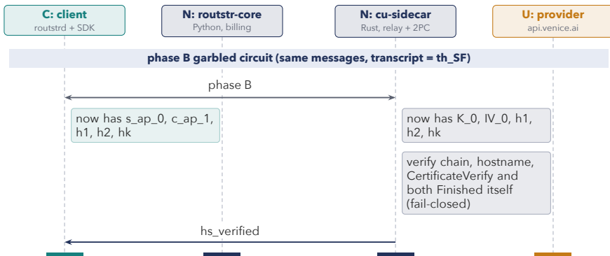
Figure 7.5: Phase B gives each party its own application keys; the sidecar then verifies the whole handshake itself.
