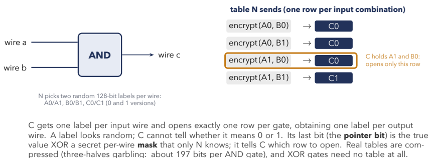
Figure 8.1: One garbled AND gate.
