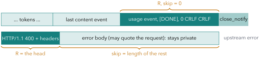
Figure 9.1: What n_C2S and n_C3S look at.
