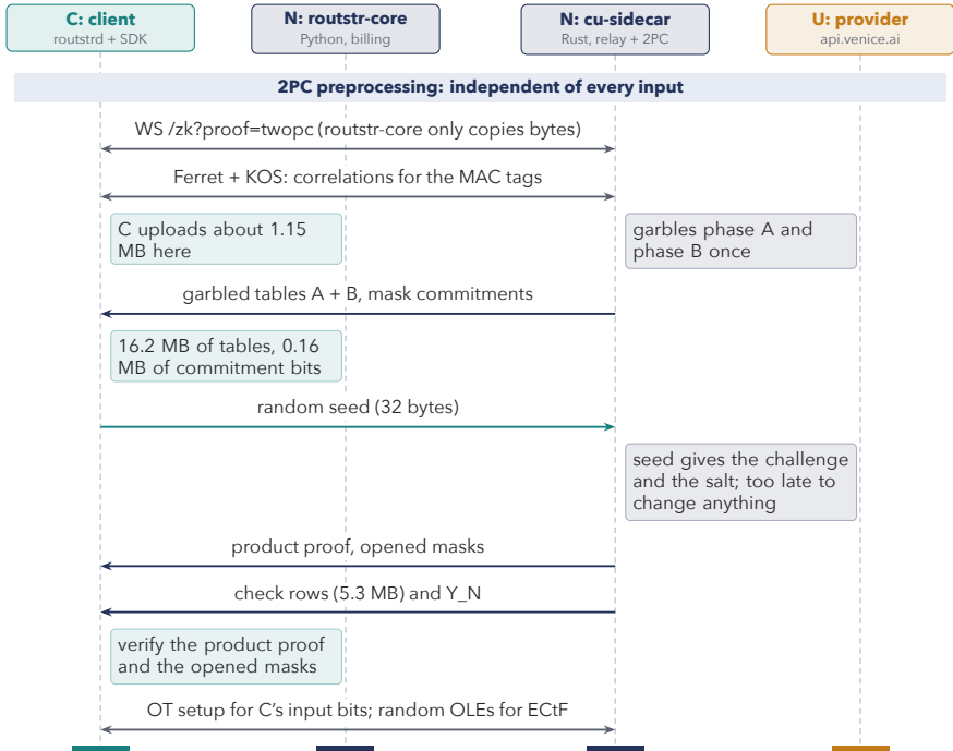
Figure 7.2: Preprocessing: the expensive, input-independent part of the 2PC. Every byte of it can happen before a request exists.
