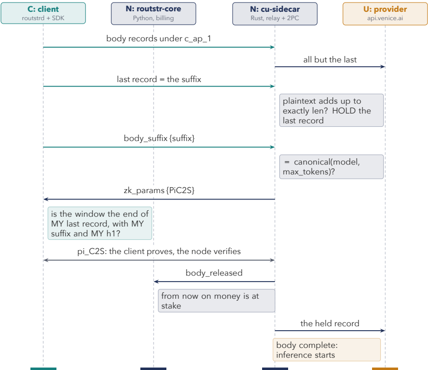
Figure 7.7: Epoch 1. The record that completes the body is held until the suffix proof verifies.
