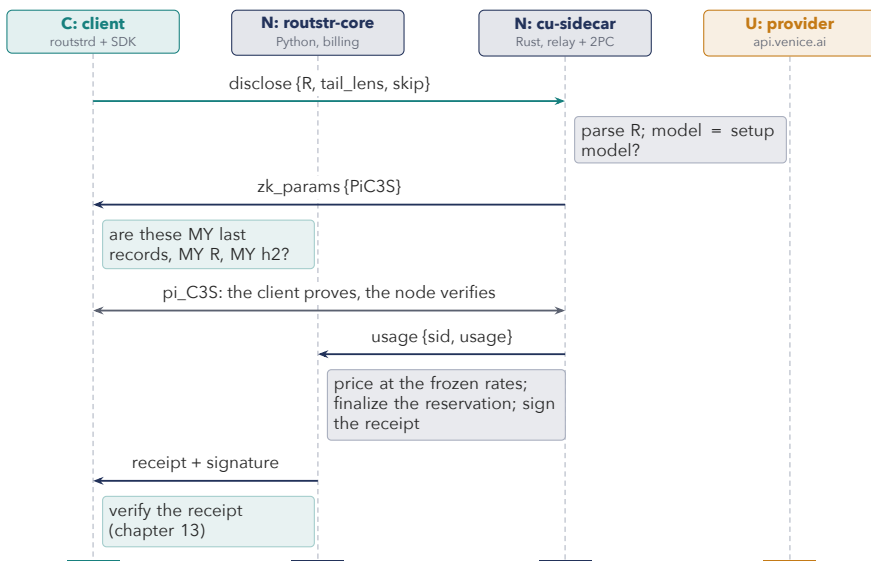
Figure 7.9: Disclosure, the usage proof and settlement.
