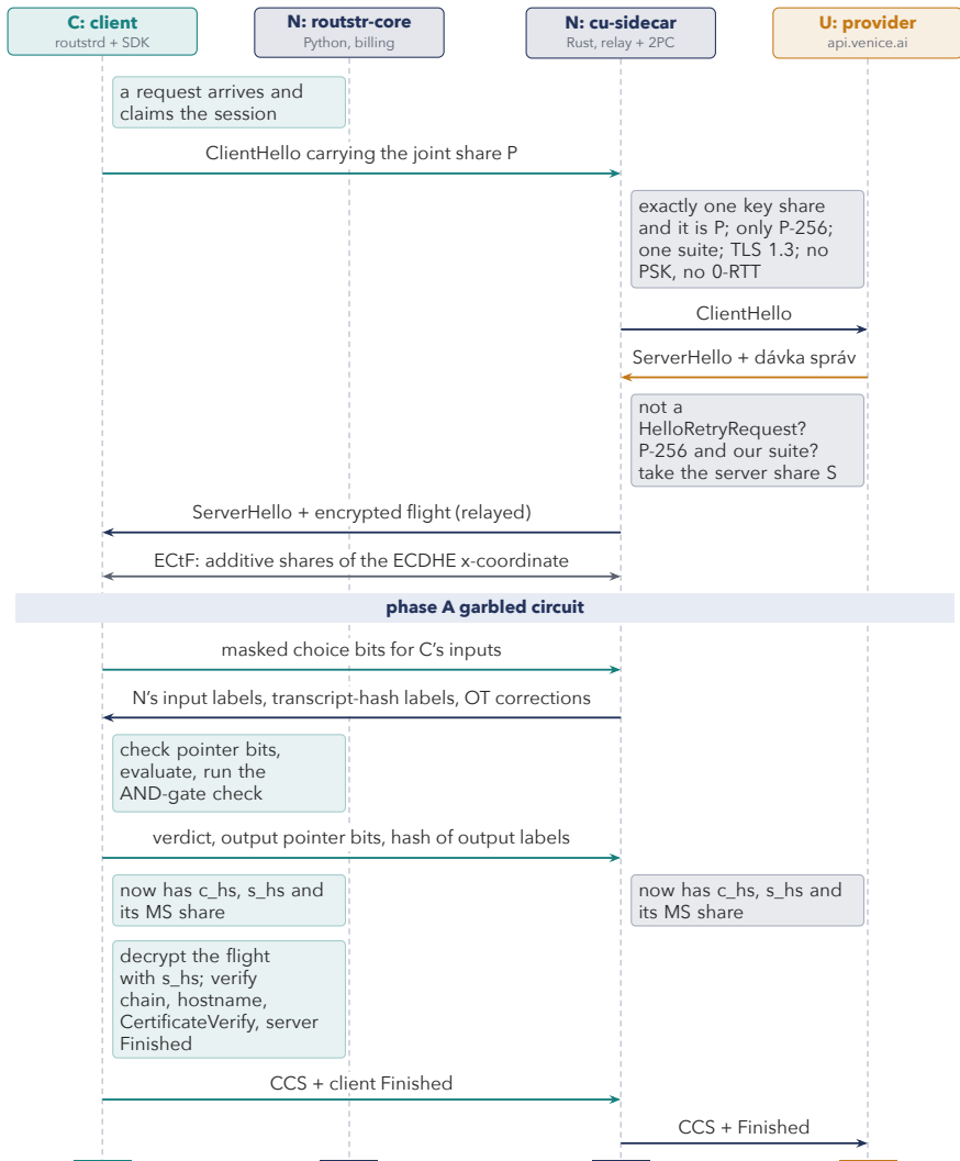
Figure 7.4: The handshake. The sidecar relays the ClientHello only if its single key share is the joint point.
