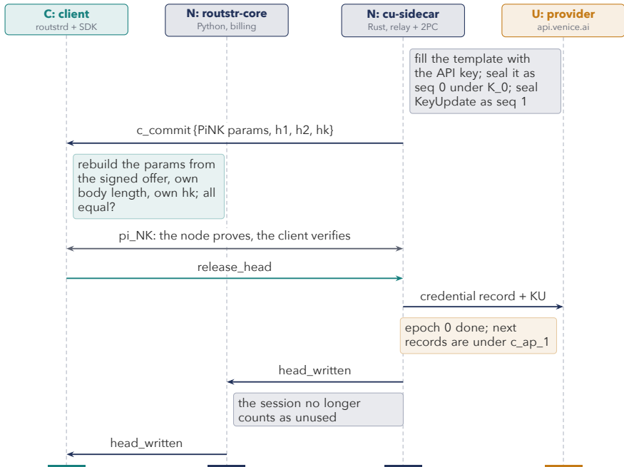
Figure 7.6: Epoch 0. The node commits to its record, proves it matches the template, and writes it only when the client says go.
