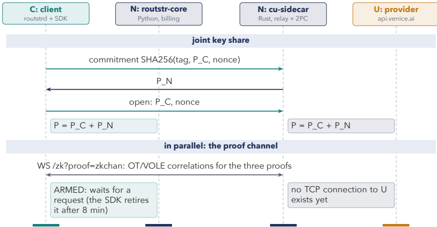
Figure 7.3: The joint key share (commit, then open) and the proof channel.
